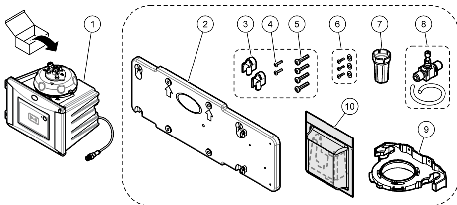
Figure 2 Product components
